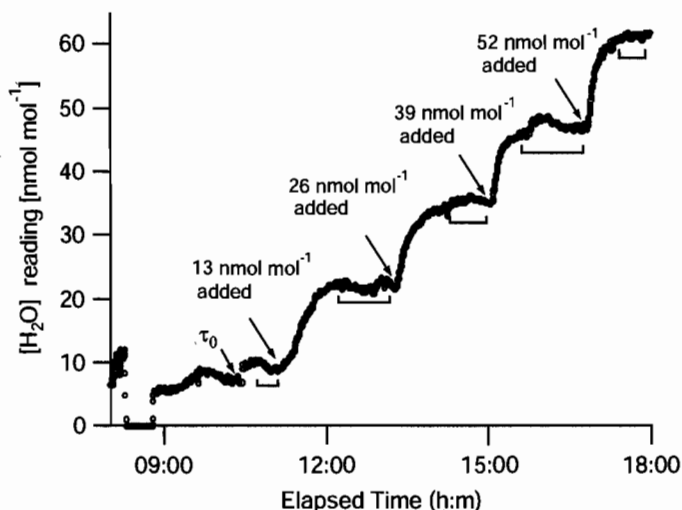
FIG. 6. Time profile showing H 2 O reading during H 2 O addition to purified PH 3 stream and the data points used to plot the response curve shown in Fig. 7.
