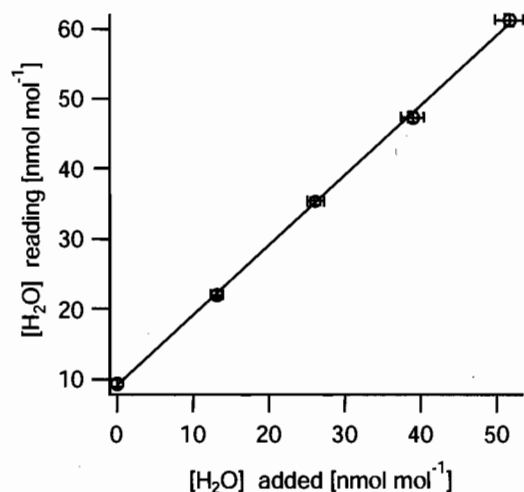
FIG. 7. Response curve for H 2 O addition to dry PH 3 calculated from data in Fig. 6.
