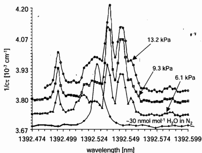
FIG. 5. Spectra of purified PH 3 at 6.1, 9.3, and 13.2 kPa and comparison with spectrum of H 2 O in N 2 at 13.2 kPa. Note: upper three spectra are offset on the vertical scale for clarity.
