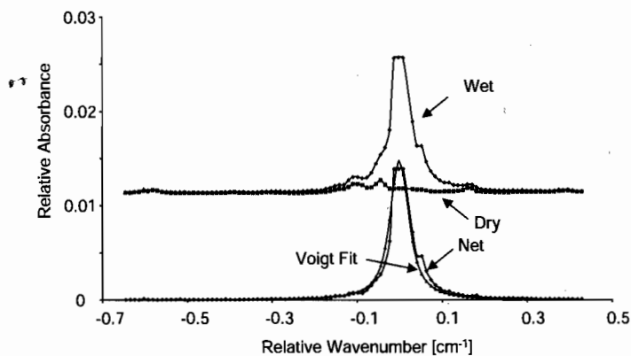
FIG. 4. Measured spectra and Voigt fit of the 1392.5 \text{ nm H}_2\text{O} line. 829 \text{ nmol mol}^{-1} of H_2O in PH_3 at a total pressure of 12.6 \text{ kPa} . For the Voigt fit, Gaussian full-width = 0.0208 \text{ cm}^{-1} , Lorentzian full-width = 0.04473 \text{ cm}^{-1} . Note: upper spectra are offset on the vertical scale for clarity.
