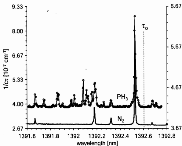
FIG. 3. Comparison of water vapor spectra in N_2 ( \sim 220 \text{ nmol mol}^{-1} ) and PH_3 ( \sim 400 \text{ nmol mol}^{-1} ). Note: upper spectra are offset on the vertical scale for clarity.
